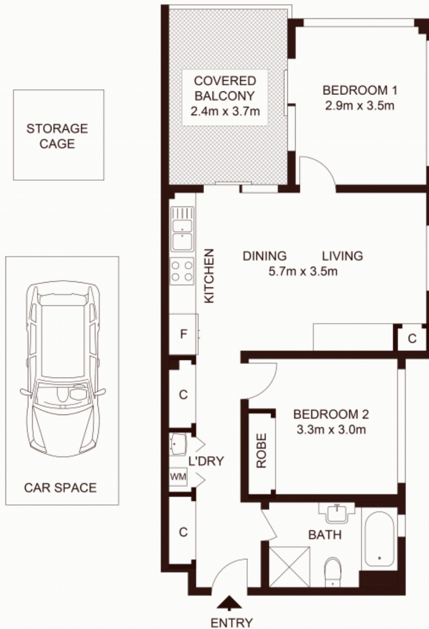
LEVEL 2
